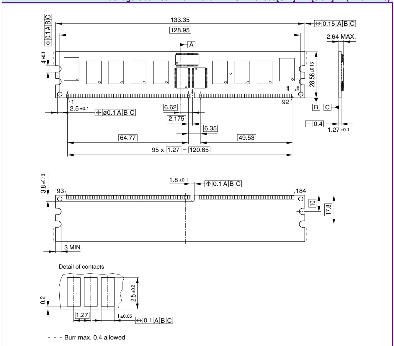
Package Outlines – Raw Card A HYS72D32300[G/H]BR-[5/6/7]-C (1 Rank × 8)
